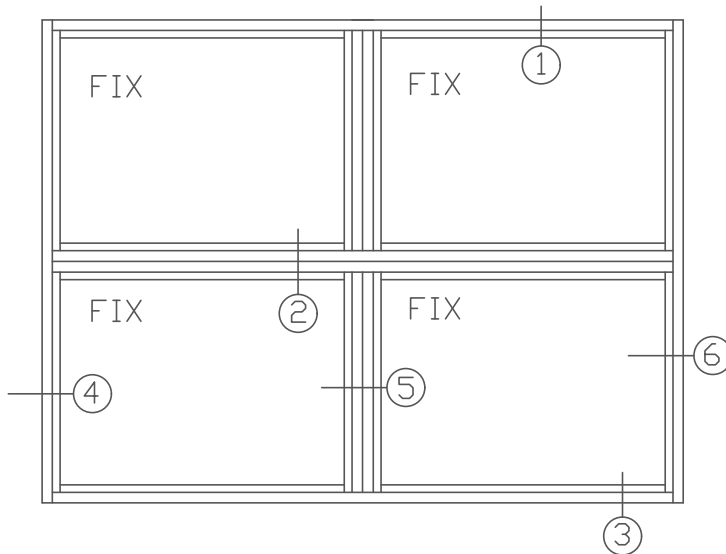
TYPICAL ELEVATION
